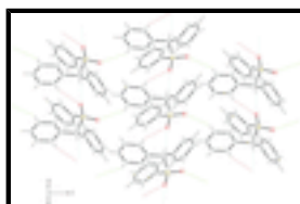
Fig. 2. Weak intermolecular hydrogen bonds of the type C–H...O leading to a two-dimensional network that propagates along the bc plane (viewing direction approximately along [110]). Color scheme for dashed lines: blue: H1...O2 contacts, red: H7...O2 contacts, green: H4...O1 contacts.
